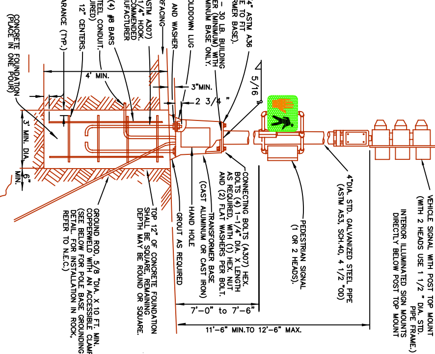
VEHICLE SIGNAL PEDESTAL (SEE PEDESTRIAN SIGNAL PEDESTAL FOR CONTROLLER MOUNTING)
